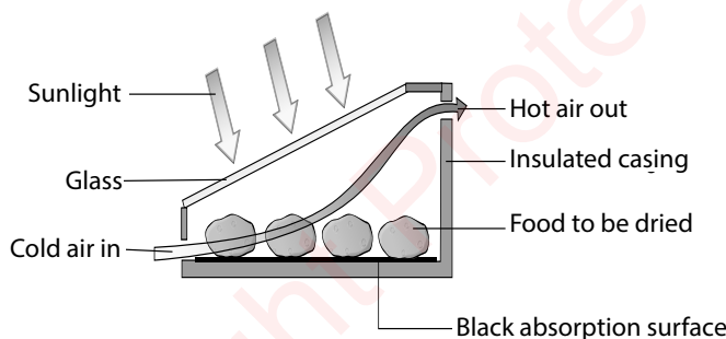
Photograph 3.4: Solar Dryer
